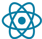
React
